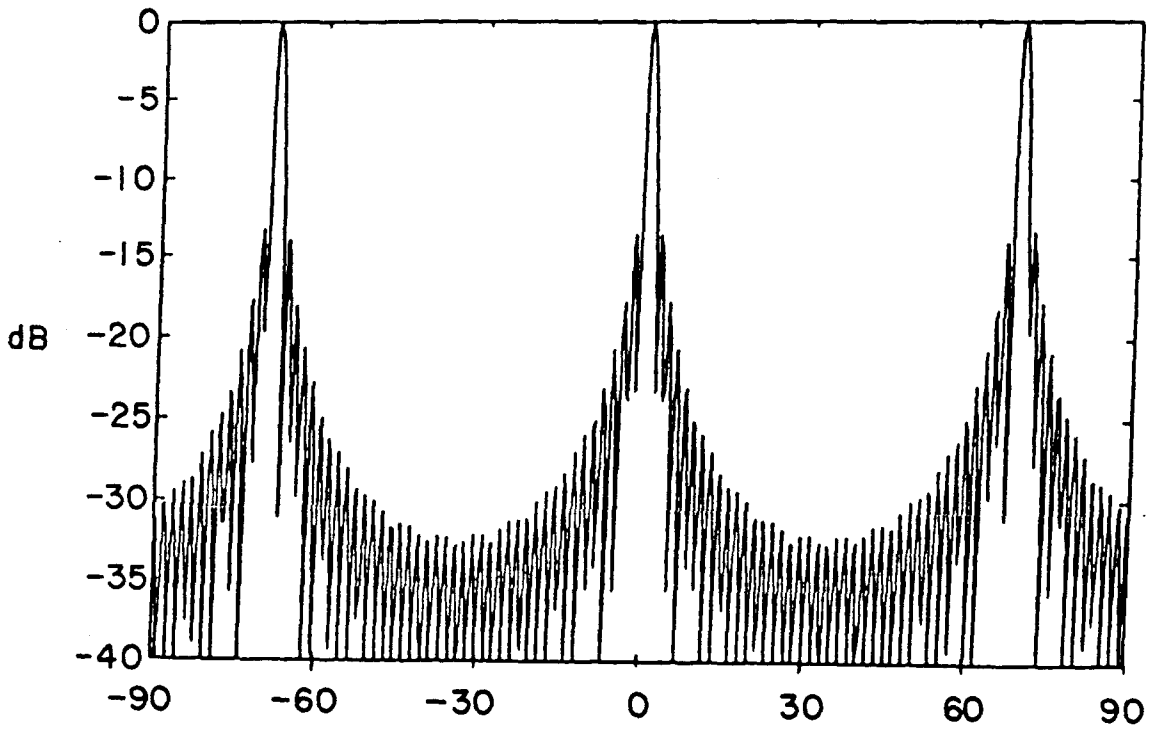
Angle theta in degrees Pattern of a thinned array antenna with uniform spacing containing grating lobes
